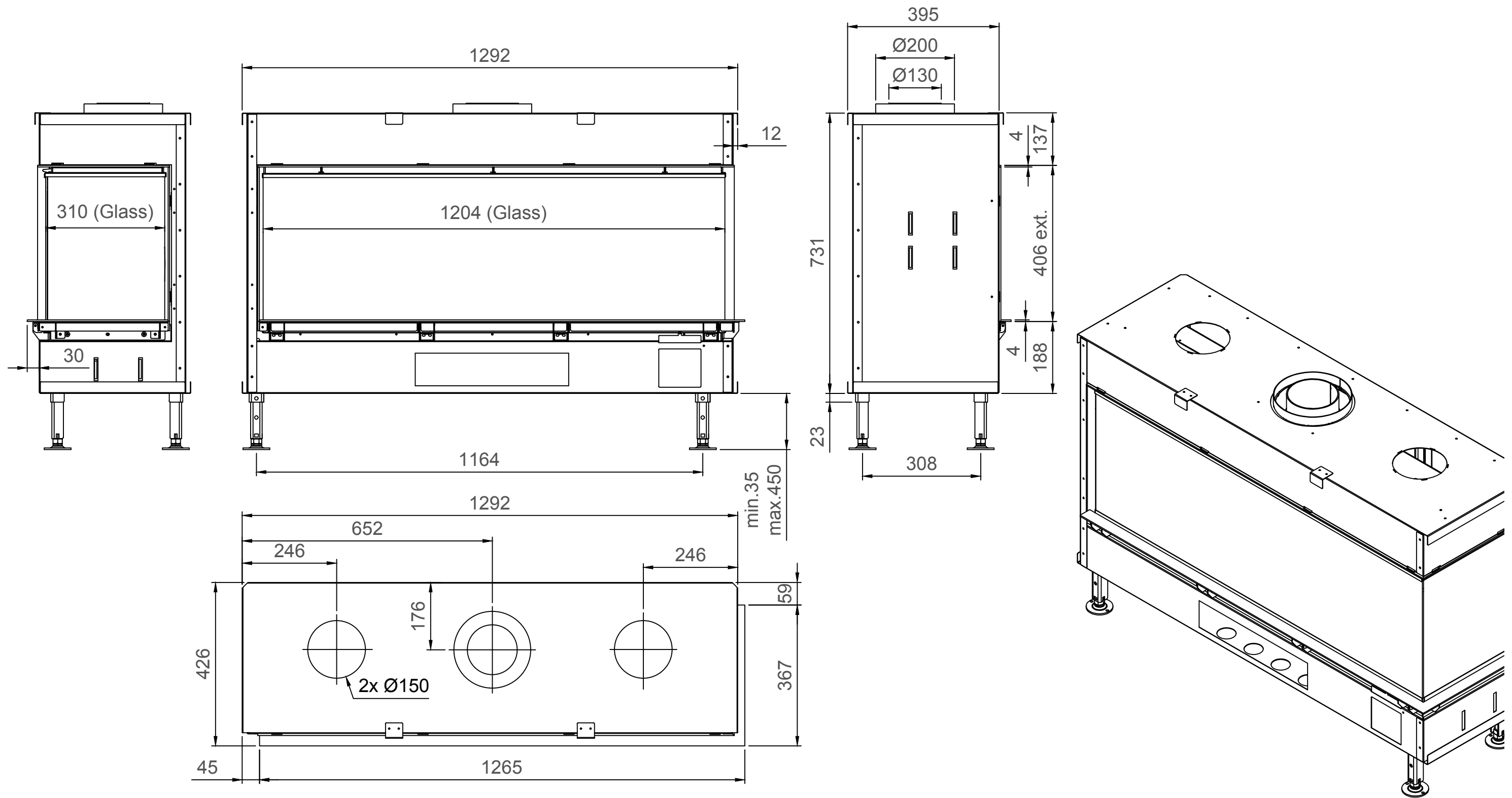
Luna Diamond 1300CR Gas/Gaz
