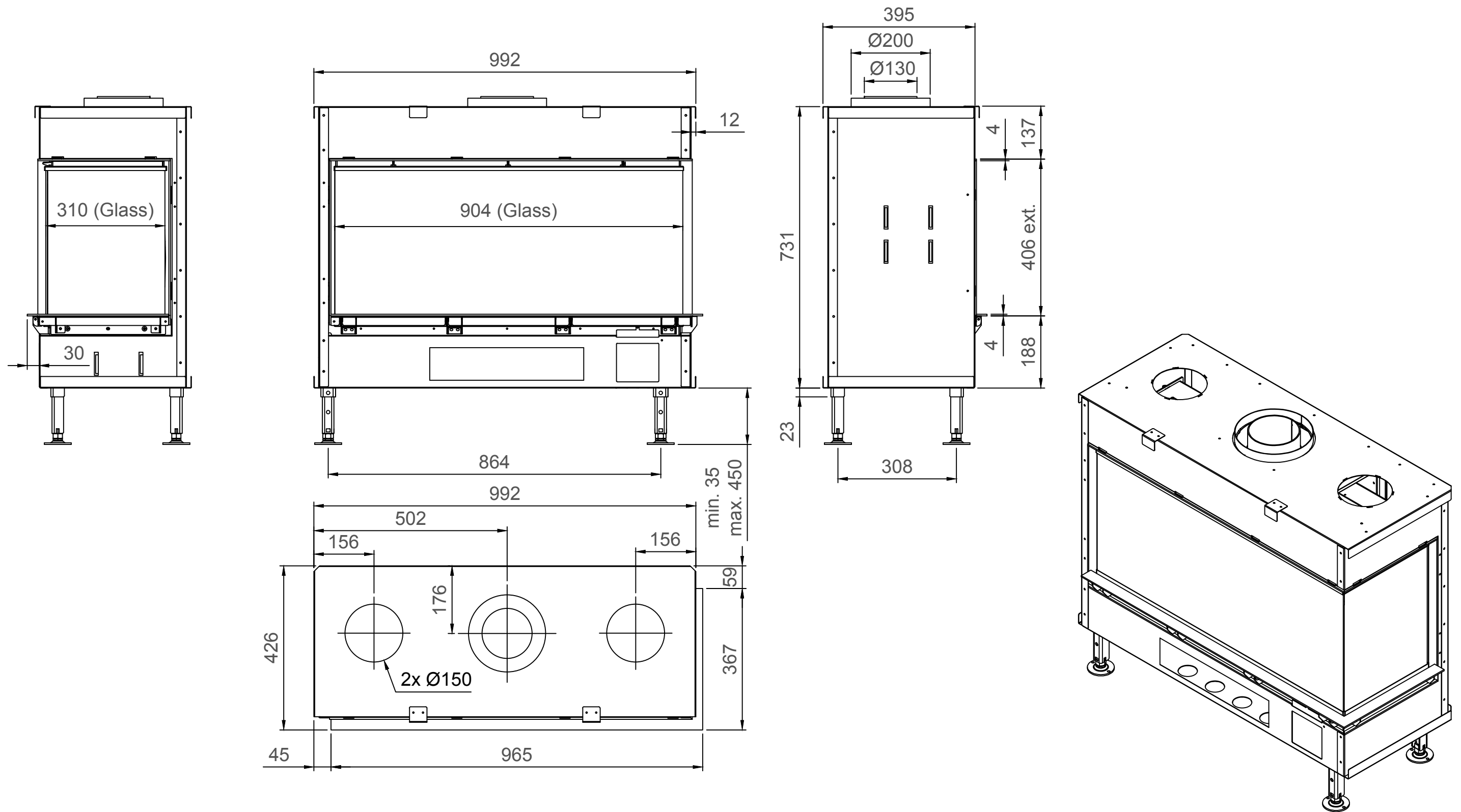
Luna Diamond 1000CR Gas/Gaz
