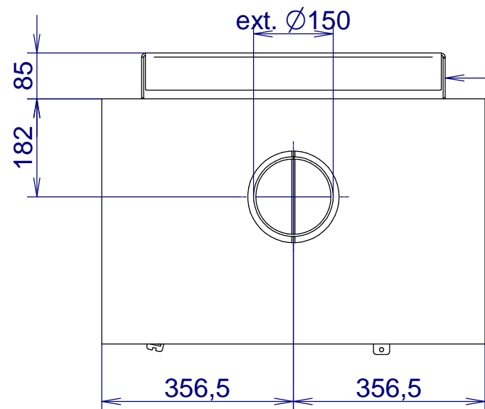
VENUS 630 V23 metal door in the box + console for wall
